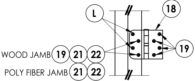
HINGE DETAIL
