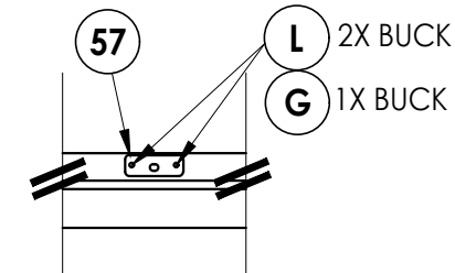
DETAIL 1 Astragal Strike Plate
